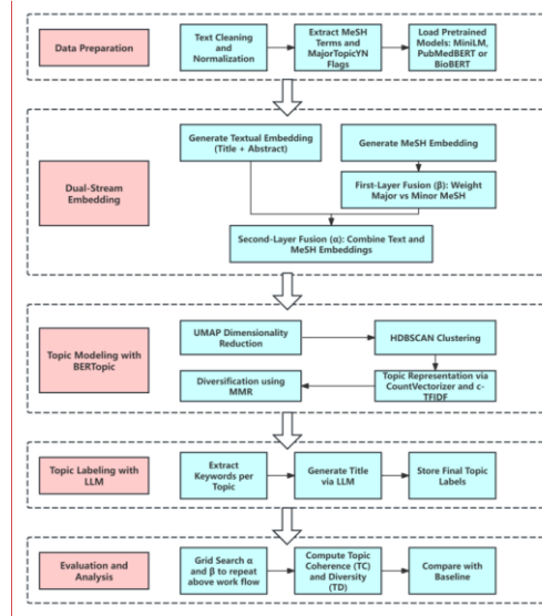
Figure 1: System workflow of the proposed dual-stream topic modelling framework.
