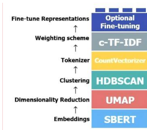
Figure 2: Modular architecture of the BERTopic pipeline.
